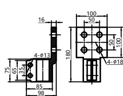
LV1(0.44kV) bushing terminal
