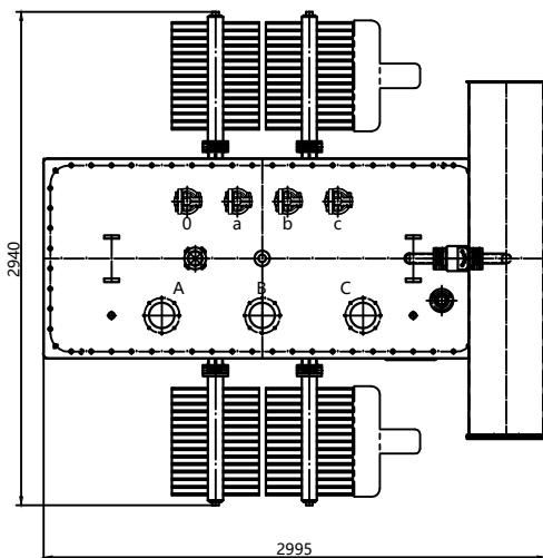
H.V bushing terminal
