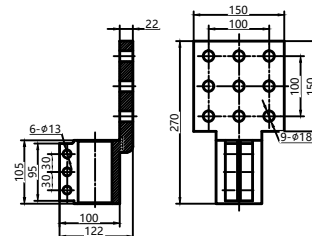
LV2(0.23kV) bushing terminal
