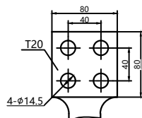
H.V bushing terminal
